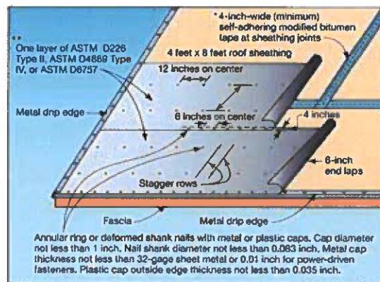
Sealed Roof Deck Option #2
