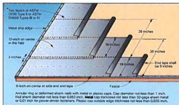
Sealed Roof Deck Option #3
